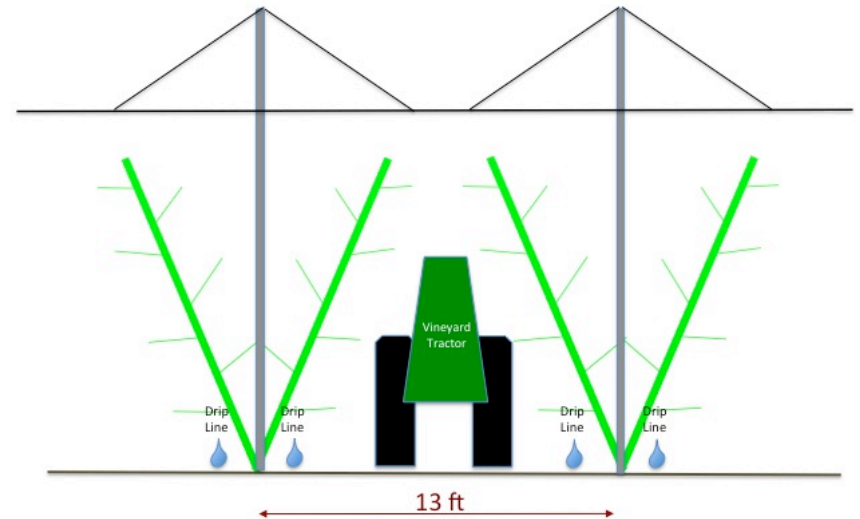
13 ft Pole-Cable Tent Covers: V-Lyre (3 ft spacing, 1116 trees/acre) or V-SSA (1.5 ft spacing, 2232 trees/acre) Angled Fruiting Walls + Tractor Sprayer
